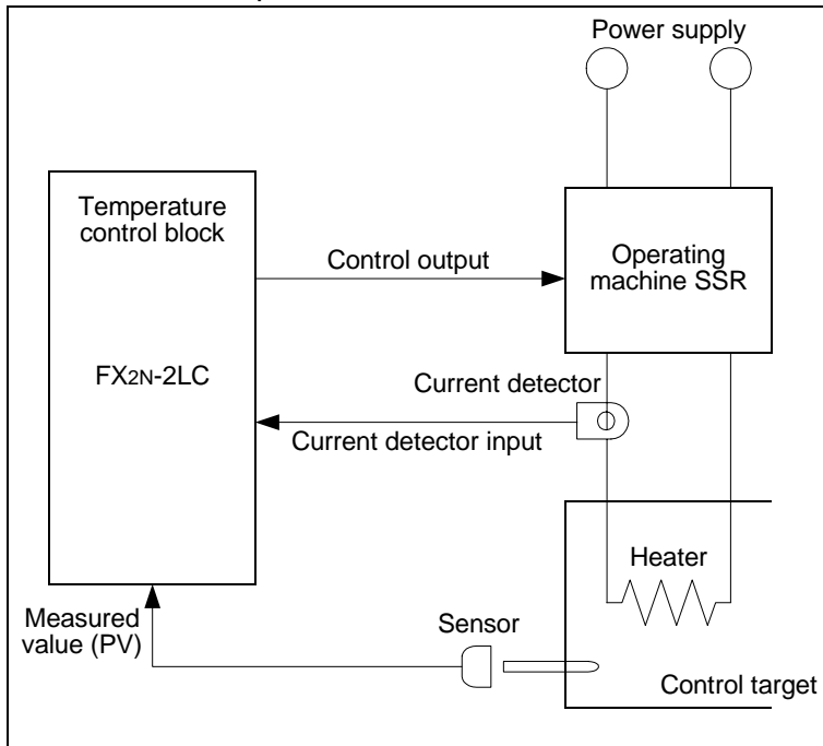
Connection example
