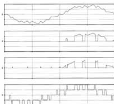
Conventional PWM
